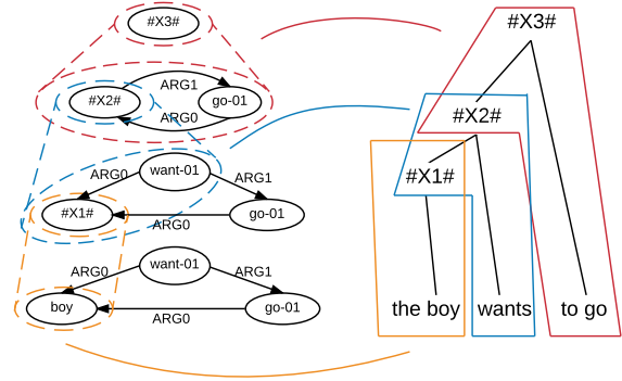
Figure 1: Graph-to-string derivation.
