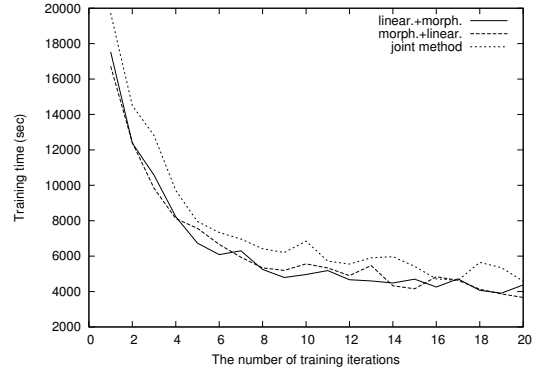
Figure 3: Training time (in seconds) by training iteration.
