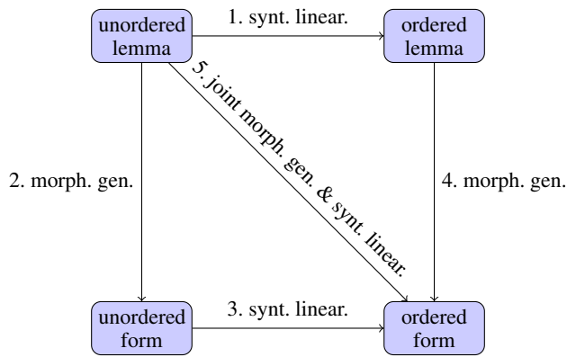
Figure 2: Several pipelines for syntactic linearization ( synt. linear. ) and morphological generation ( morph. gen. ).
