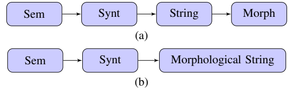
Figure 1: (a) NLG pipeline based on the meaning text theory (Bohnet et al. 2010), (b) pipeline of this paper. Sem stands for Semantics, Synt stands for syntax and Morph stands for morphology.
